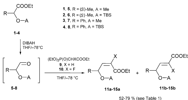
Scheme 1. HWE synthesis of 2-fluoroalkenoates from protected \alpha -hydroxy aldehydes.
