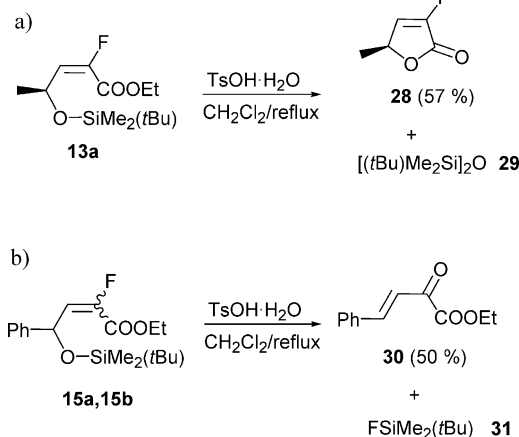
Scheme 3. The result of acid-catalysed deprotection of 4-alkyl(phenyl)-2-fluoroalkenoates with TsOH·H 2 O: a) cyclisation; b) defluorination and allyl rearrangement of the \pi system.
