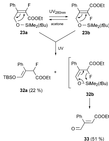
Scheme 4. Photoinduced isomerisation and defluorination of 3-phenyl-2-fluorobut-2-enoates.
