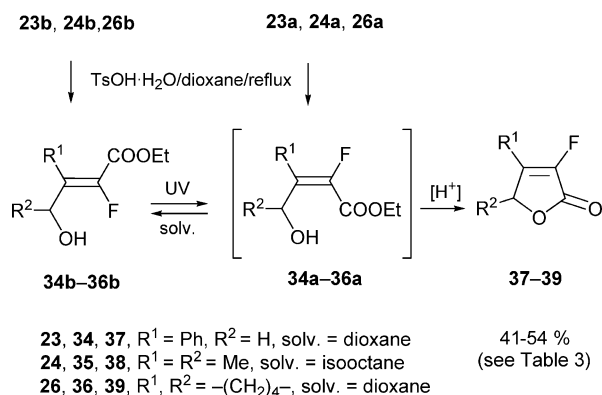
Scheme 5. Photoisomerisation and cyclisation of 2-fluoro-4-hydroxy-but-2-enoates.
