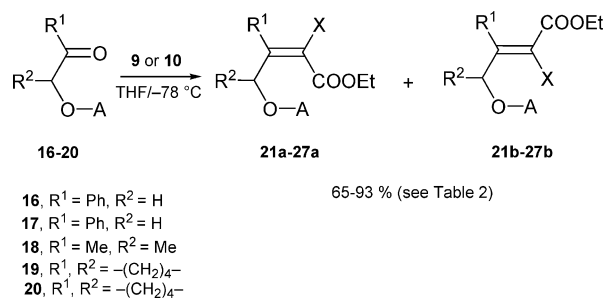
Scheme 2. HWE synthesis of 2-fluoroalkenoates from protected \alpha -hydroxy ketones.
