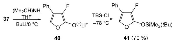
Scheme 6. Synthetic exploitation of 2-fluorobutenolides.
